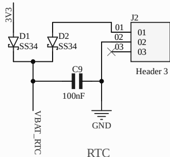
RTC
