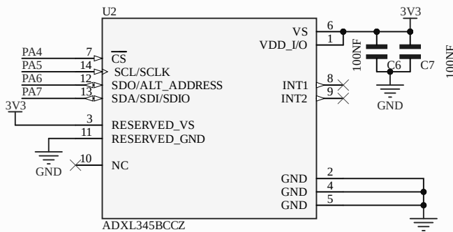
ADXL345BCCZ
