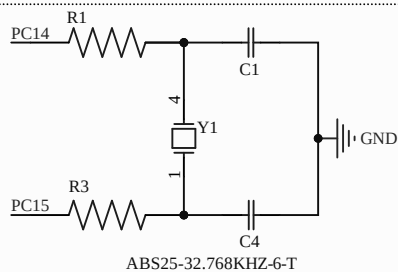
ABS25-32.768KHZ-6-T
