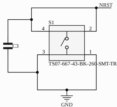
Reset Switch
